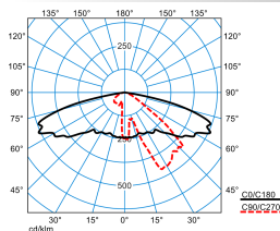
Publisca P1W-AB2L-LRA/1800-730 2G1S
