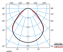
ValineoG5 M84 PW19 38-50/4ML-830 ETDD (stage 3)
