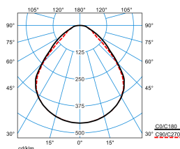
ValineoG5 M84 PW19 38-50/4ML-830 ETDD (stage 4)
