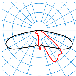
Publisca P2-AB2L/2600-740 3G1S ETDD (CLO end value) TX300600 ■ C0 - C180 ■ C90 - C270 DIN 5040: A30 UTE: 1,00 l DLOR: 100 % ULOR: 0 % CEN Flux Code: 34 71 96 100 100
