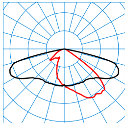
LIQ 70N-AB7L-SLR1/9100-730 10G1 ET (CLO end value) TX278148 ■ C0 - C180 ■ C90 - C270 DIN 5040: A30 UTE: 1,00 E DLOR: 100 % ULOR: 0 % CEN Flux Code: 39 76 98 100 100
