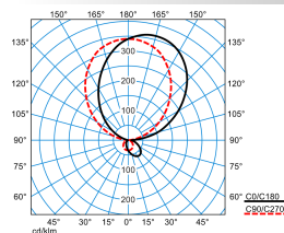
Sanesca W3-S1/R LED5000-840 ET 01
