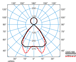
SFlow H2-L MRX LED6400-830 ETDD 03 TX721324
