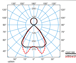
SFlow H2-L MRX LED6400-830 ETDD 03 TX770407
