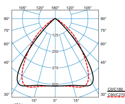
ELINE HE LN60-160 ML 830 L225 0 20
