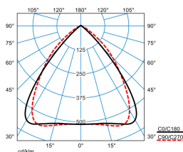
ELINE HE LN60-160 ML 830 L225 4 20
