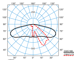
Publisca P2-AB2L/1650-740 2G1S ETDD (CLO initial value) TX301452 DIN 5040: A30 UTE: 1,00 G DLOR: 100 % ULOR: 0 % CEN Flux Code: 34 70 96 100 100
