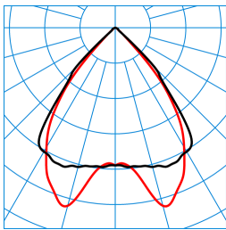
SFlow D1-L MRX LED3200-840 ET 03 TX769884
