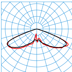
Publisca P2-RB6L-LRA/2400-730 3G1S ET (CLO initial value) TX301569 ■ C0 - C180 ■ C90 - C270 DIN 5040: A20 UTE: 1,00 J DLOR: 100 % ULOR: 0 % CEN Flux Code: 20 57 98 100 100
