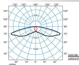
LIQ 50N-SB3L-LR/1650-740 2G1 ET (CLO initial value)
