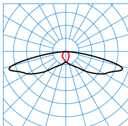
LIQ 50N-SB3L-LR/1650-740 2G1 ET (CLO end value) TX776295 ■ C0 - C180 ■ C90 - C270 DIN 5040: A30 UTE: 1,00 l DLOR: 100 % ULOR: 0 % CEN Flux Code: 31 64 92 100 100
