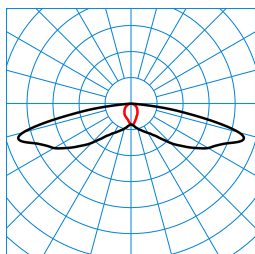
LIQ 50N-SB3L-LR/1650-740 2G1 ET (CLO initial value) TX776296 ■ C0 - C180 ■ C90 - C270 DIN 5040: A30 UTE: 1,00 l DLOR: 100 % ULOR: 0 % CEN Flux Code: 31 64 92 100 100
