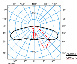
Publisca P2-AB2L-LRA/1800-730 2G1S ET (CLO initial value) TX301381 DIN 5040: A30 UTE: 1,00 G DLOR: 100 % ULOR: 0 % CEN Flux Code: 34 70 96 100 100
