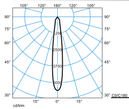
E-Line PRO 78 BV G2 RF-SP 50-835 M34 ETBLE 03 03
