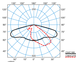
LIQ 70N-AB7L-LR/9100-740 10G1 ET(CLO end value)
