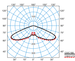
Publisca P2-RB6L-LR/4200-740 6G1S ET (CLO initial value) TX301105
