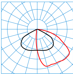
Inveria C 210 AM21R/3900-840 ETBLE +CAS TX774847
