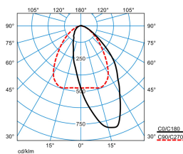
7850 HE LAN120 840 L225 4 50
