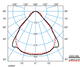
SFlow D2-L MRW LED4000-8TW ETDD8 03 (DSU) TX877008
