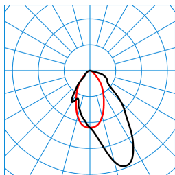
CreavoAct M57 LWW-03 42-8 ETDD8 01(ACTDCW) TX775910 ■ C0 - C180 ■ C90 - C270 DIN 5040: A50 UTE: 1,00 C DLOR: 100 % ULOR: 0 % CEN Flux Code: 70 92 99 100 100
