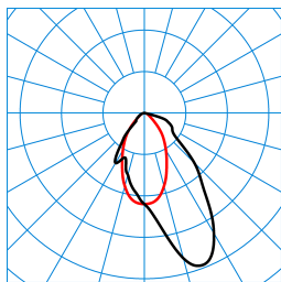
CreavoAct M57 LWW-03 42-8 ETDD8 01(ACTDSU) TX775911 ■ C0 - C180 ■ C90 - C270 DIN 5040: A50 UTE: 1,00 C DLOR: 100 % ULOR: 0 % CEN Flux Code: 70 92 99 100 100
