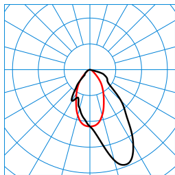
CreavoAct M57 LWW-03 42-8 ETDD8 01(ACTDWW) TX775912 ■ C0 - C180 ■ C90 - C270 DIN 5040: A50 UTE: 1,00 C DLOR: 100 % ULOR: 0 % CEN Flux Code: 70 92 99 100 100
