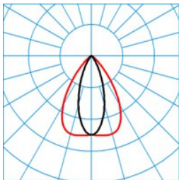
ELINE FL HE LVN40 865 L150 3 20
