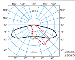
LIQ 50N-AB2L-LR/6800-722 6G1 ET (CLO initial value)
