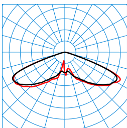
Publisca P1-RB6L-LR/2600-740 3G1S ET (CLO initial value) TX300917 ■ C0 - C180 ■ C90 - C270 DIN 5040: A20 UTE: 1,00 J DLOR: 100 % ULOR: 0 % CEN Flux Code: 20 57 98 100 100
