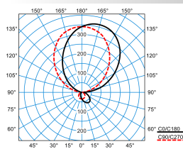
Sanesca W3 LED5000-830 ET 01
