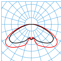
Publisca P1W-RBT-LR/3200-740 4G1S ET (CLO initial value) TX301336 ■ C0 - C180 ■ C90 - C270 DIN 5040: A20 UTE: 0.99 l + 0.01 T DLOR: 99 % ULOR: 1 % CEN Flux Code: 26 63 91 99 100 0 0 0 1
