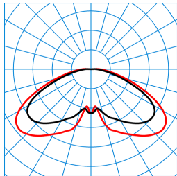
Publisca P1W-RBT-LR/3200-740 4G1S TX053576 ■ C0 - C180 ■ C90 - C270 DIN 5040: A20 UTE: 0.99 l + 0.01 T DLOR: 99 % ULOR: 1 % CEN Flux Code: 26 63 91 99 100 0 0 0 1
