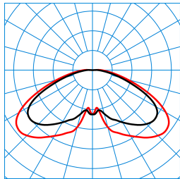
Publisca P1W-RBT-LR/3200-740 4G1S ET (CLO end value) TX301279 ■ C0 - C180 ■ C90 - C270 DIN 5040: A20 UTE: 0.99 l + 0.01 T DLOR: 99 % ULOR: 1 % CEN Flux Code: 26 63 91 99 100 0 0 0 1
