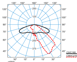
Publisca P2-AB2L/2900-730 4G1S ETDD (CLO end value)
