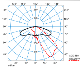
Publisca P2-AB2L/2900-730 4G1S ETDD (CLO initial value)
