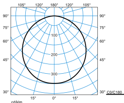
Olisq RWD3 DW 30-8TW ETBLE +CAS-S IP54 + RWD3 ZDR 1/1 03 (DWW)
