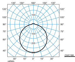
Olisq RWD3 DW 30-8TW ETBLE +CAS-S IP54 (DSU) TX873823
