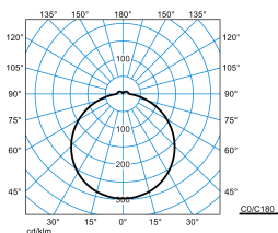
Olisq RWD3 DW 30-8TW ETBLE +CAS-S IP54 + RWD3 ZDR 1/2 01 (DWW)
