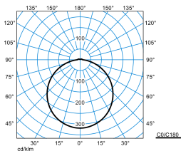
Olisq RWD3 DW 30-8TW ETBLE +CAS-S IP54 + RWD3 C 01 (DWW)
