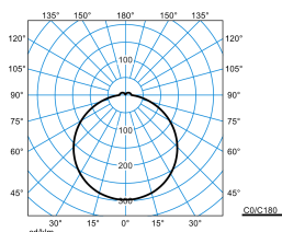
Olisq RWD3 DW 30-8TW ETBLE +CAS-S IP54 + RWD3 ZDR 1/2 03 (DWW) TX873842
