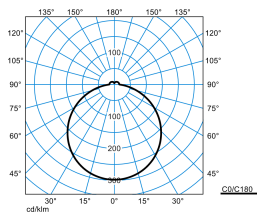
Olisq RWD3 DW 30-8TW ETBLE +CAS-S IP54 (DCW) TX873822
