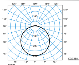
Olisq RWD3 DW 30-8TW ETBLE +CAS-S IP54 (DWW) TX873824
