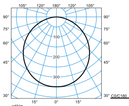
Olisq RWD3 DW 30-8TW ETBLE +CAS-S IP54 + RWD3 ZDR 1/1 05 (DWW)
