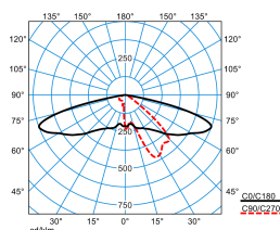
Publisca P1W-AB2L-LR/2600-740 3G1S
