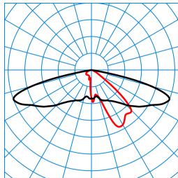
Publisca P1W-AB2L-LR/2600-740 3G1S TX053484 ■ C0 - C180 ■ C90 - C270 DIN 5040: A30 UTE: 1,00 l DLOR: 100 % ULOR: 0 % CEN Flux Code: 32 69 96 100 100 0 33 67 0
