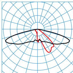
Publisca P1W-AB2L-LR/2600-740 3G1S ET (CLO initial value) TX301420 ■ C0 - C180 ■ C90 - C270 DIN 5040: A30 UTE: 1,00 l DLOR: 100 % ULOR: 0 % CEN Flux Code: 32 69 96 100 100 0 33 67 0
