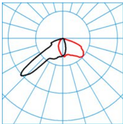
Jovie 70-FL1L-8-91-740-CLO-B
