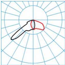
Jovie 70-FL1L-8-91-740-CLO-E
