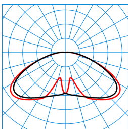
Publisca P1W-RBT-LRA/1800-740 2G1S ET (CLO initial value) TX300504 ■ C0 - C180 ■ C90 - C270 DIN 5040: A20 UTE: 0.97 l + 0.03 T DLOR: 97 % ULOR: 3 % CEN Flux Code: 26 63 91 97 100 4 16 28 3
