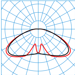
Publisca P1W-RBT-LRA/1800-740 2G1S TX053582 ■ C0 - C180 ■ C90 - C270 DIN 5040: A20 UTE: 0.97 l + 0.03 T DLOR: 97 % ULOR: 3 % CEN Flux Code: 26 63 91 97 100 4 16 28 3
