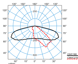
LIQ 50N-AB2L-LR/5600-727 6G1 ET (CLO end value)
