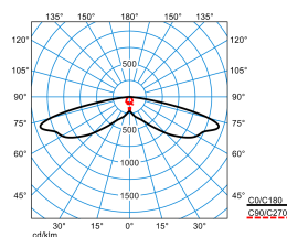
Publisca P1-SB3L/800-730 2G1S ETDD (CLO initial value)
