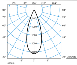
78 SNS L37 RH1-05/05 SRFL 8-940 ETDD 05
