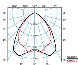
ELINE HE LW60-160 ML 830 L225 0 20
