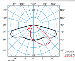
LIQ 70N-AB7L-SLR2/9100-727 10G1 ET(CLO initial value)
