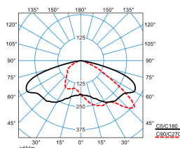
9711SG-AB7L-LRA/51/62/75-740 8G2 (7500 lm)
