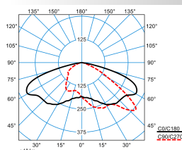
9711SG-AB7L-LRA/51/62/75-740 8G2 (5100 lm)
