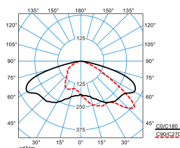
9711SG-AB7L-LRA/51/62/75-740 8G2 (6200 lm)
