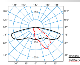
9301K AB2L-SLR1/4600-740 8G3 ET(CLO initial value)
