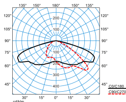
9311 AB7L-SLR3/3500-740 4G3 ET(CLO end value)
