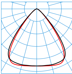
SFlow C2-L LW19 4000-830 ET 01 TX768661
