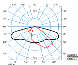
LIQ 70N-AB7L-LRA/7500-722 8G1 ETDD (CLO end value)
