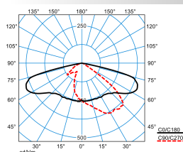
LIQ 70N-AB7L-LRA/7500-722 8G1 ETDD (CLO initial value)
