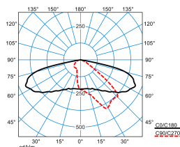
LIQ 50N-AB2L-LRA/2600-722 4G1 ETDD (CLO initial value) TX776051
