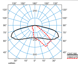
LIQ 50N-AB2L-LRA/2600-722 4G1 ETDD (CLO end value) TX776050
