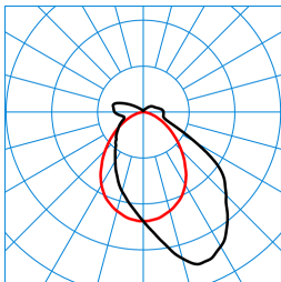
TugraHE Act 12 PAW 50-840 ETDD8 01 (ACTDSU) TX302752 ■ C0 - C180 ■ C90 - C270 DIN 5040: B40 UTE: 0.87 E + 0.13 T DLOR: 87 % ULOR: 13 % CEN Flux Code: 48 79 93 87 100 7 25 60 13
