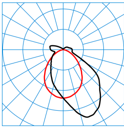
TugraHE Act 12 PAW 50-840 ETDD8 01 (ACTDWW) TX303560 ■ C0 - C180 ■ C90 - C270 DIN 5040: B40 UTE: 0.87 E + 0.13 T DLOR: 87 % ULOR: 13 % CEN Flux Code: 48 79 93 87 100 7 25 60 13
