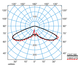
Publisca P1-RB6L/2200-730 3G1S ETDD (CLO end value) TX301402 DIN 5040: A20 UTE: 1,00 J DLOR: 100 % ULOR: 0 % CEN Flux Code: 20 57 98 100 100
