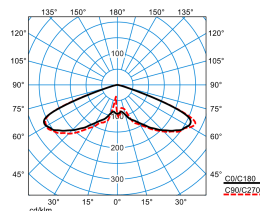
Publisca P1-RB6L/2200-730 3G1S ETDD (CLO end value)
