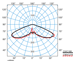
Publisca P1-RB6L/2200-730 3G1S ETDD (CLO initial value) TX301183 DIN 5040: A20 UTE: 1,00 J DLOR: 100 % ULOR: 0 % CEN Flux Code: 20 57 98 100 100
