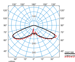
Publisca P1-RB6L/2200-730 3G1S ETDD (CLO initial value)
