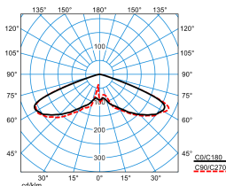
Publisca P2-RB6L-LR/2600-740 3G1S ET (CLO initial value) TX300935 DIN 5040: A20 UTE: 1,00 J DLOR: 100 % ULOR: 0 % CEN Flux Code: 20 57 98 100 100
