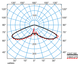
Publisca P2-RB6L-LR/2600-740 3G1S ET (CLO end value) TX300438 DIN 5040: A20 UTE: 1,00 J DLOR: 100 % ULOR: 0 % CEN Flux Code: 20 57 98 100 100
