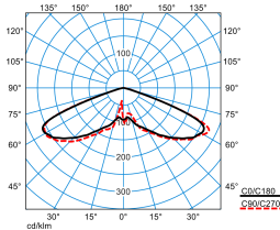
Publisca P2-RB6L-LR/2600-740 3G1S TX047863 DIN 5040: A20 UTE: 1,00 J DLOR: 100 % ULOR: 0 % CEN Flux Code: 20 57 98 100 100
