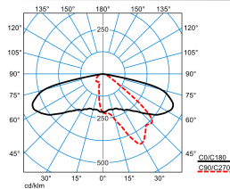
Cuvia60-AB2L8S3-82-740-ET-CAB-26 (CLO initial value)
