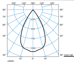
E-Line PRO 78 BV G2 RF-VFL 20-M+F M53 ETBLE 03 Blank
