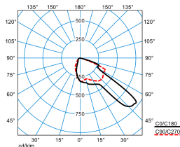
LIQ 50N-FR1L/4200-722 4G1 ET (CLO end value) TX780556
