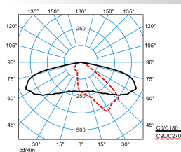
LIQ 50N-AB2L-LRA/2400-727 4G1 ETDD (CLO initial value)
