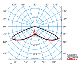
Publisca P1W-RB6L/2200-740 3G1S ETDD (CLO end value)
