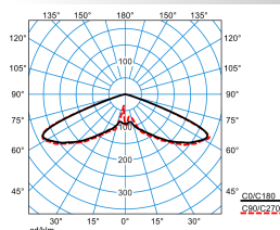
Publisca P1W-RB6L/2200-740 3G1S ETDD (CLO initial value)
