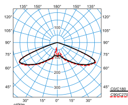
Publisca P1W-RB6L/2200-740 3G1S
