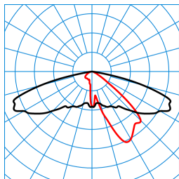
Publisca P1W-AB2L-LRA/4600-740 6G1S ET (CLO initial value) TX300993 ■ C0 - C180 ■ C90 - C270 DIN 5040: A30 UTE: 1,00 G DLOR: 100 % ULOR: 0 % CEN Flux Code: 34 72 97 100 100 0 0 0 0
