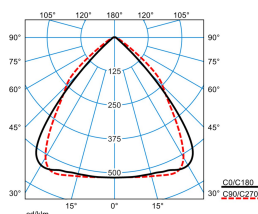
ELINE HE LW2260-160 ML 865 L225 2 50
