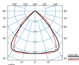
ELINE HE LW2260-160 ML 865 L225 0 50
